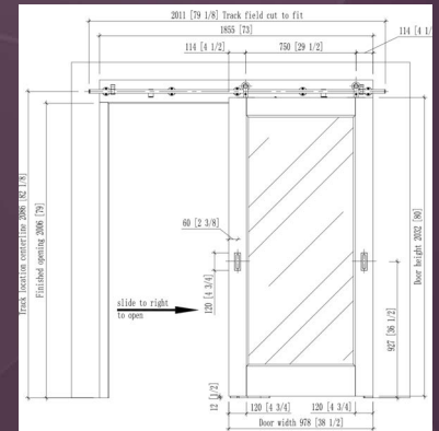
TECH DRAWING
